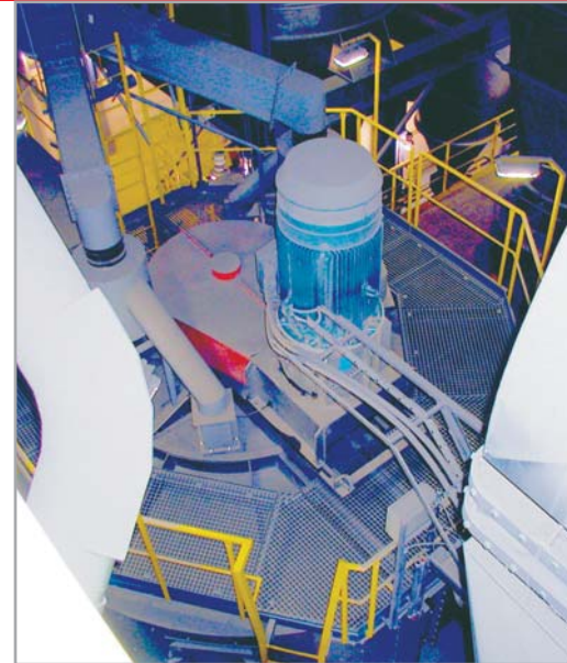
Air separator VTP 2700 at the cement grinding plant with a capacity of 80t/h – CEMMAC Horné Srnie, Slovakia
