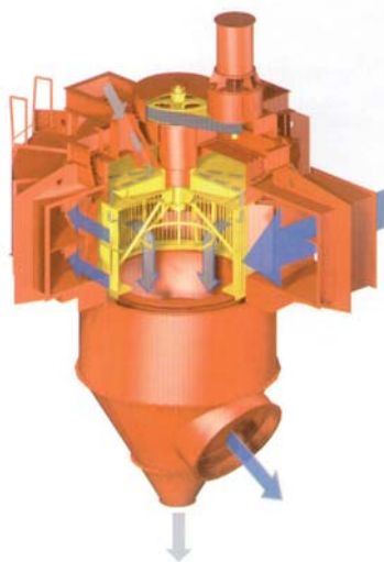
3D model of VTP air separator
