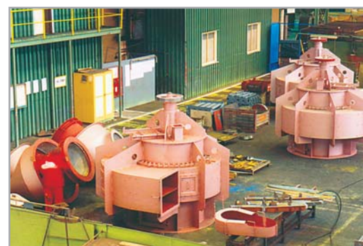
Assembly of VTP 1500 air separators for a cement grinding plant in Brazil
